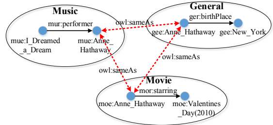
Figure 1: Three KBs should be used to answer the question “Which songs are performed by person who was born in New York and played a role in Valentine’s Day?”.
