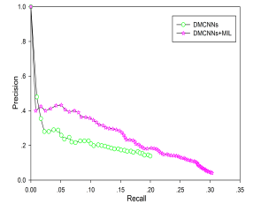
Figure 8: P-R curves for argument classification.
