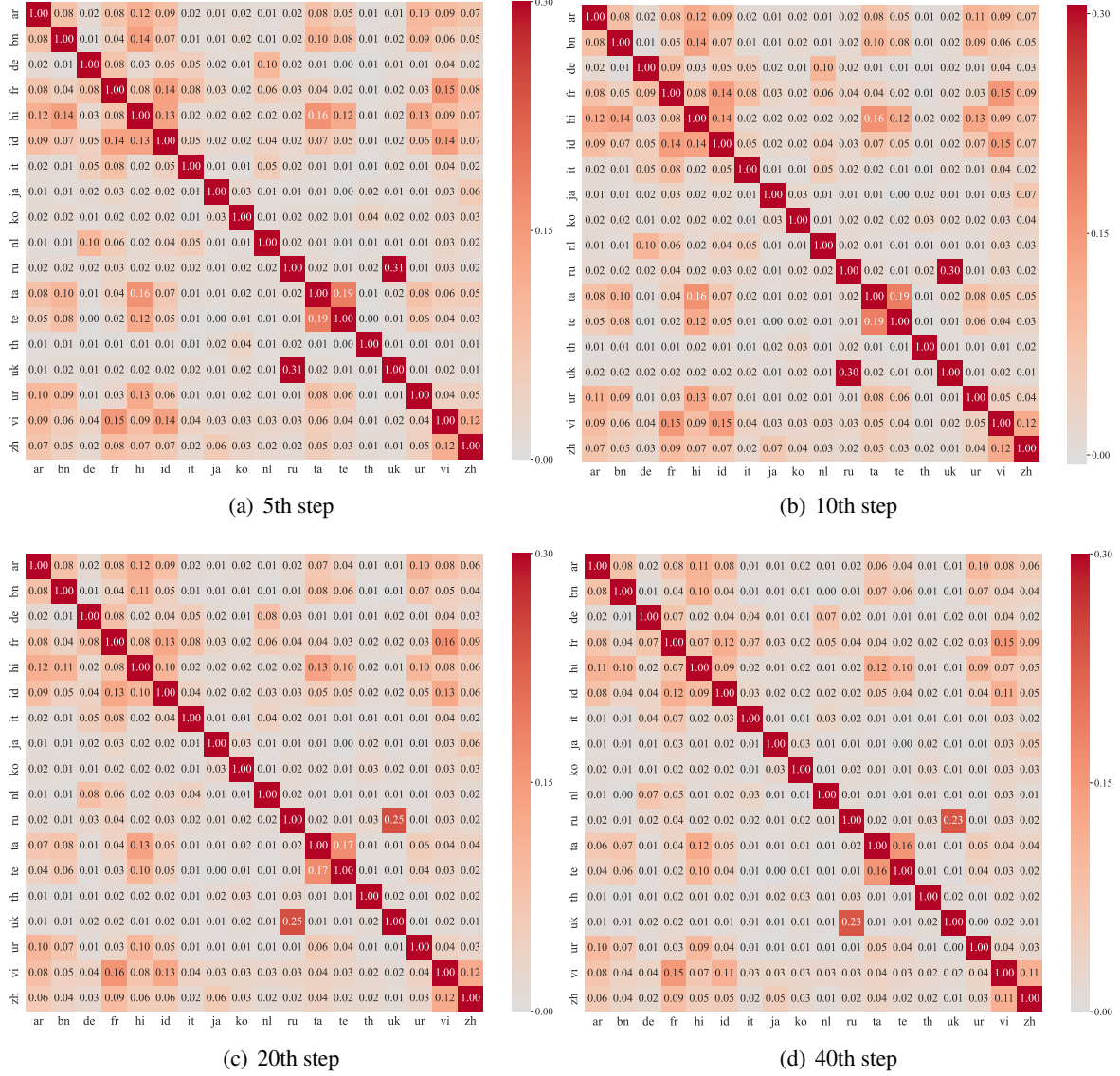
Figure 9: The language similarity matrices calculated by the parameter derivation at different fine-tuning steps using BLOOM 560M .
