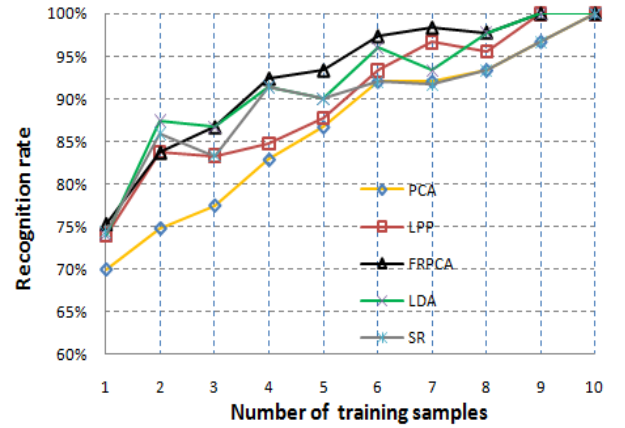
Figure 3. Accuracy rate variation of different algorithms with different number of training samples per subject.
